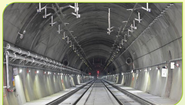
ROCS Erection in Tunnel T-50, USBRL Project
